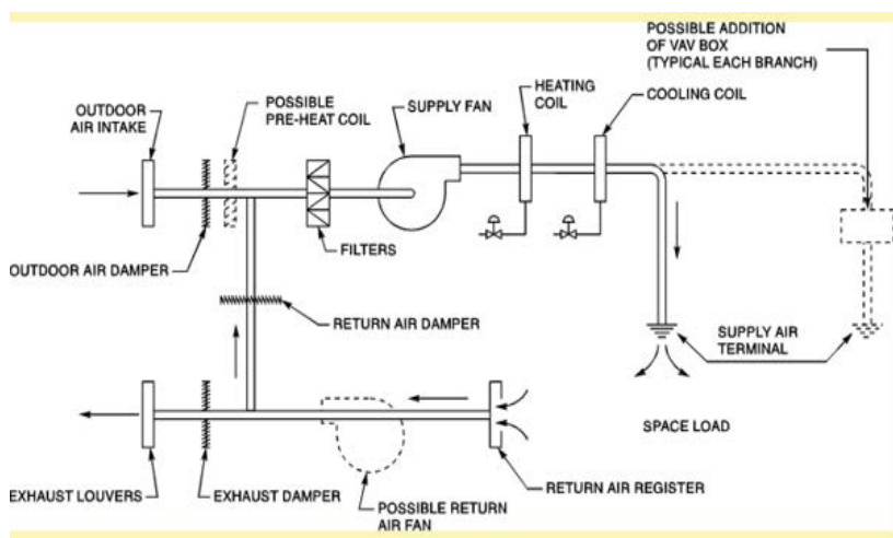
Figure 1: Schematic of a single zone HVAC system. (Courtesy of General Physics Strategies, https://www.gpstrategies.com )
